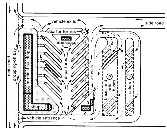
10 Large transit station with attached parking area
